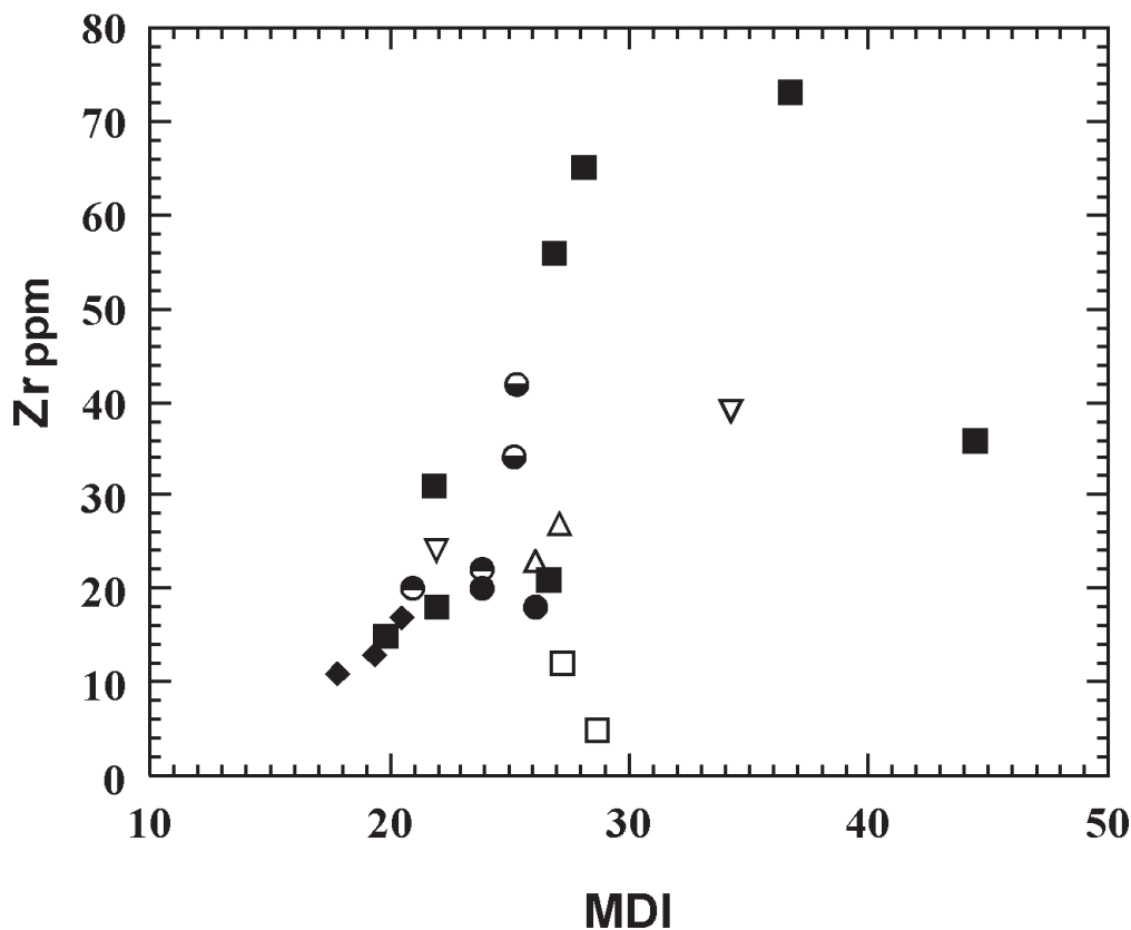
Fig. 3. Zr vs. MDI diagram. Symbols as in Fig. 2. Modified differentiation index (MDI) is calculated from the CIPW normative mineral composition (Gruenewaldt, 1973). MDI = \text{quartz} + \text{orthoclase} + \text{albite} + \text{diopside}^* + \text{ferrosilite} + \text{fayalite} + \text{nepheline} + \text{leucite} , in which \text{diopside}^* = 1.88052 \times (\text{ferrosilite of diopside}) .
