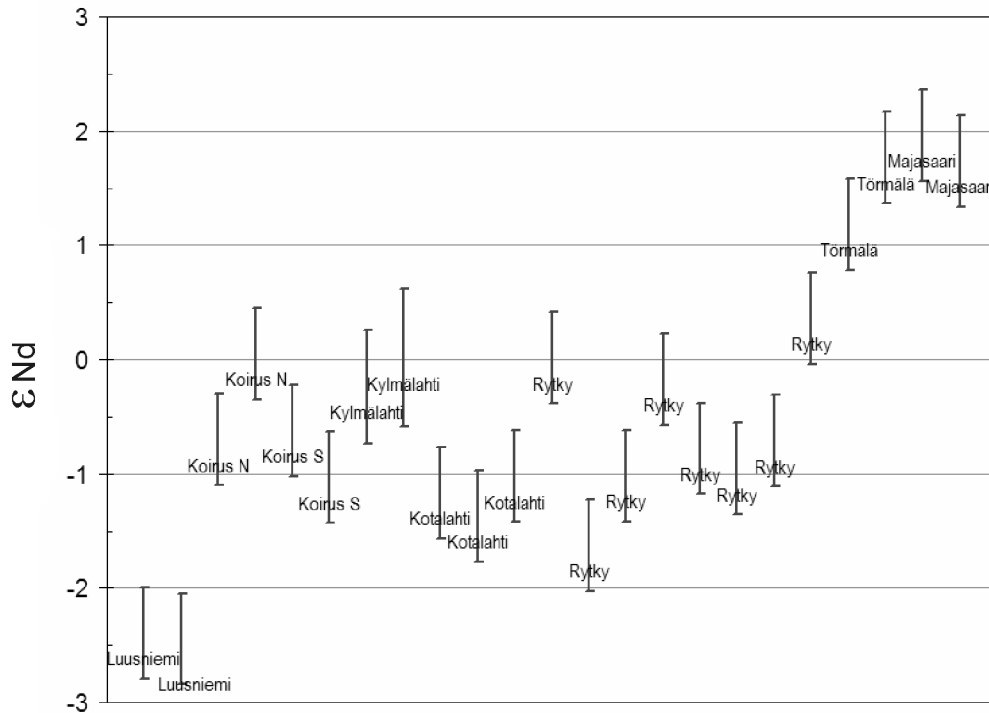
Fig. 6. \epsilon_{Nd} values for each sample calculated at 1880 Ma. The Luusniemi intrusion is located closest to the exposed main Archaean domain, while the Törmälä and Majasaari intrusions are located furthest away. Other intrusions lie within the transition zone between the Archaean and Proterozoic rocks. Error bars are 2-sigma.
