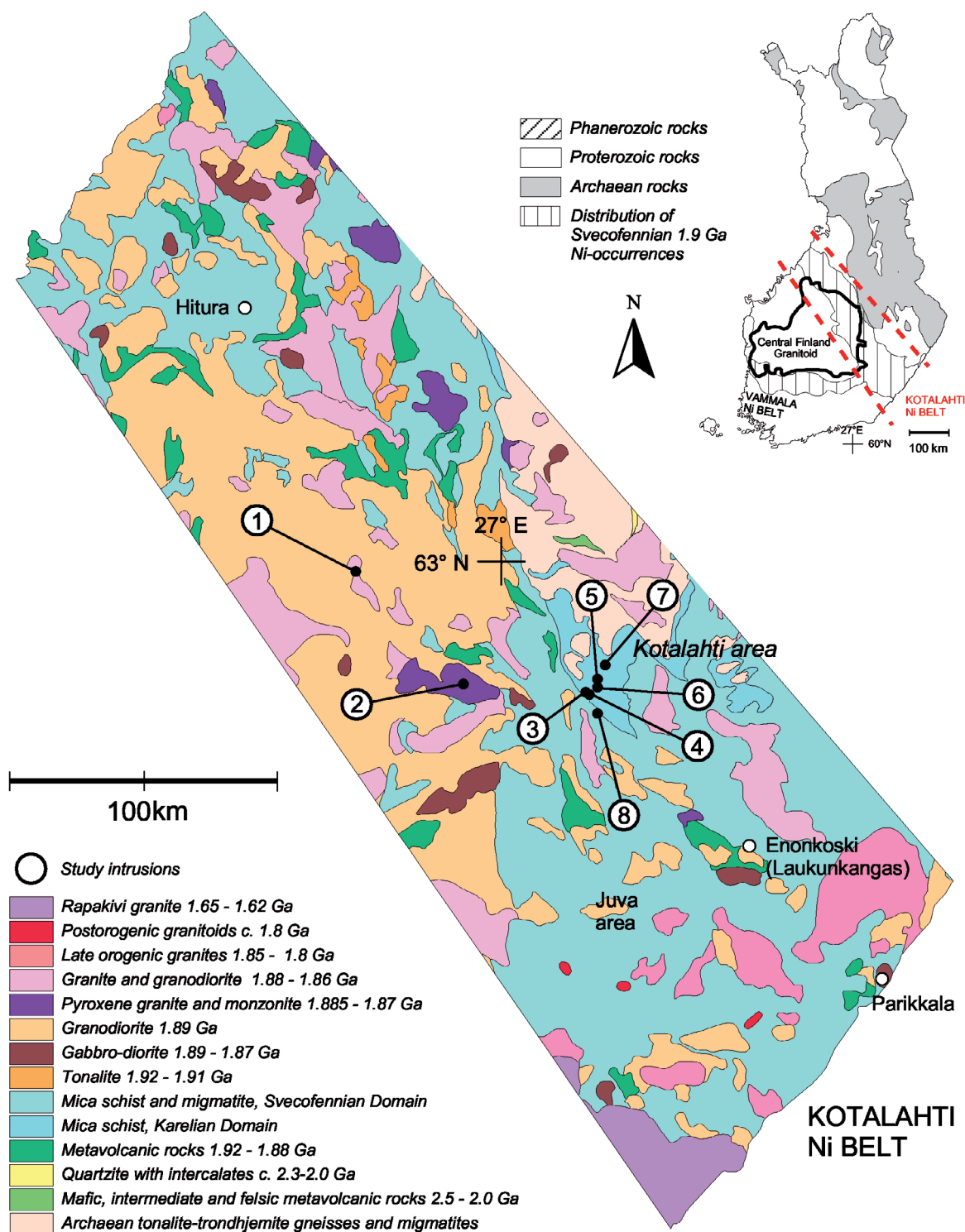
Fig. 1. Location and lithologies in the Kotalahti Nickel Belt in Finland. Studied intrusions indicated by the numbers: 1 = Majasaari, 2 = Törmälä, 3 = Kotalahti, 4 = Rytty, 5 = Koirus N, 6 = Koirus S, 7 = Luusniemi, 8 = Kylmälahti. Lithological maps simplified after Korsman et al. (1997). Hitura, Enonkoski and Parikkala Ni deposits and the Juva area also shown.
