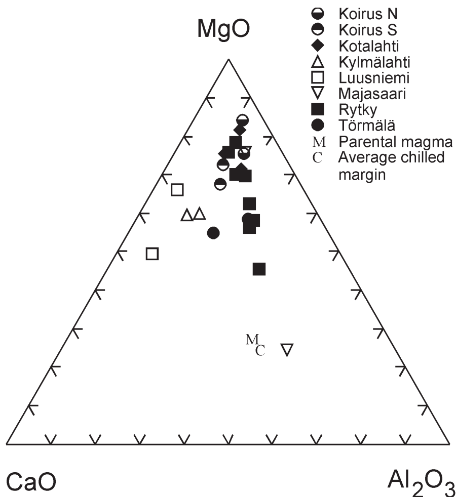
Fig. 2. CMA diagram for the studied samples. Parental magma and chilled margin compositions are from Table 2. Mineralized intrusions indicated by a closed symbol, intermediate intrusions by a half closed symbol and barren intrusions by an open symbol.
